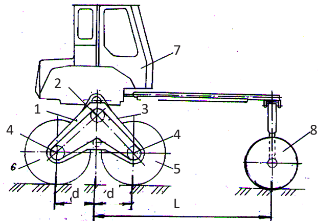
Fig. Schematic diagram of the adaptive self-propelled chassis.
