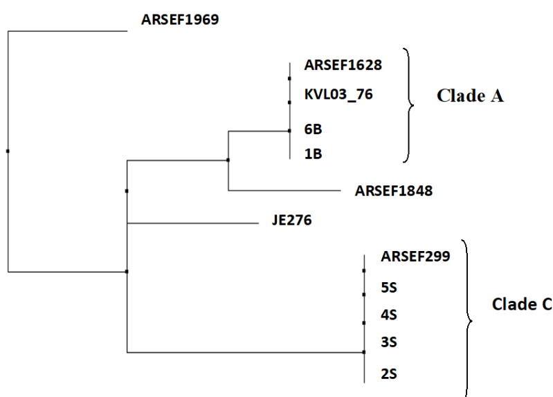
Fig.4. Elongation factor-1a (EF1- \alpha ) phylogeny of Beauveria bassiana (B1, B6, S2, S3, S4, S5) Constructed Neighbour Joining tree using PID(Waterhouse et al 2009). The GenBank accession used for the analyses are Beauveria bassiana samples: AY531896(ARSEF 1628), EF193188 (KVL 03-76), AY531904(ARSEF 1848), EF193181(KVL 03-114), DQ376244(JE276), EF193192(KVL 03-91), AY531921, (ARSEF 292)AY531923(ARSEF 299), AY531907(ARSEF1969).
