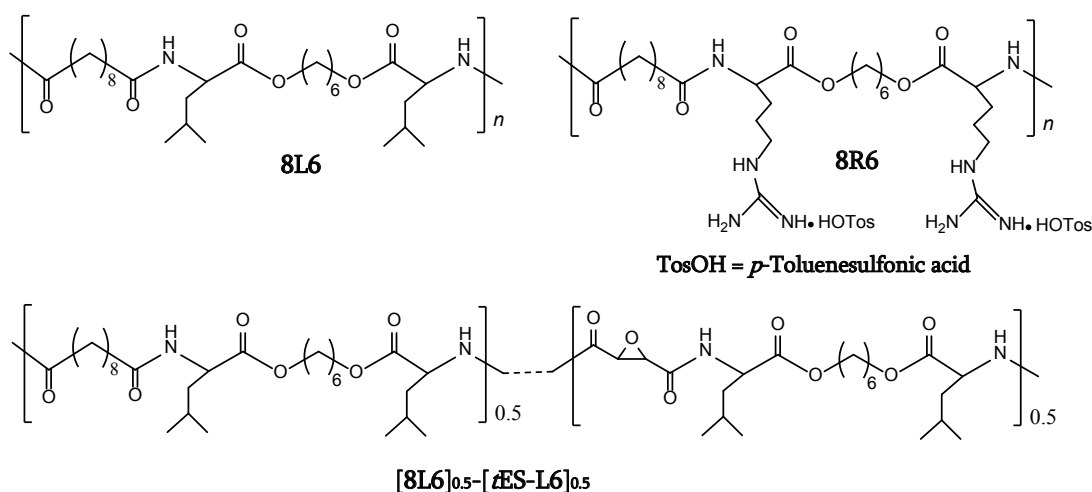
Fig. 1. The chemical structures of the PEAs used for NPs fabrication: PEA 8L6, cationic PEA 8R6, and epoxy-co-PEA [8L6]_{0.5} - [tES-L6]_{0.5} - a precursor of the new surfactant/ PEGylating agent PEG-co-PEA.
